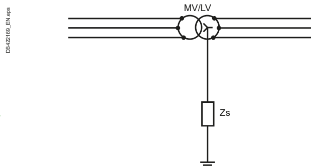
Fig. E11 IT system (impedance-earthed neutral)
