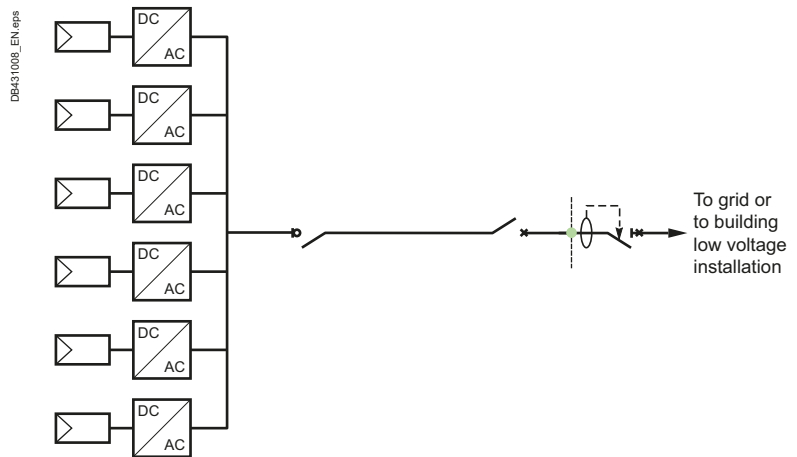
Fig. P21 Exemple of architecture based on "PV AC modules"
