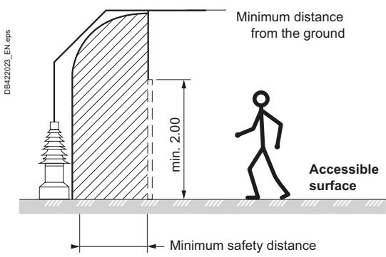
Fig. B14 Protection by installation of barriers. The safety distances are fixed by IEC 61936
