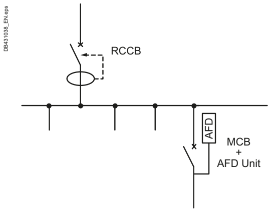
Fig. F92 AFDD unit with MCB
