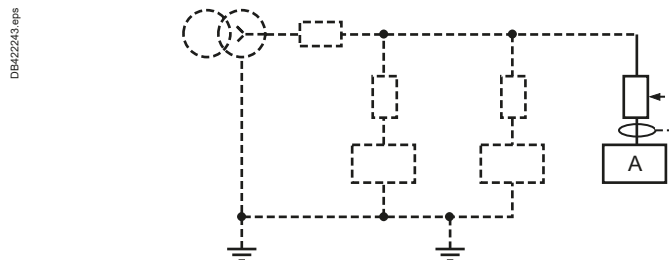
Fig. F17 Unearthed exposed conductive parts (A)
