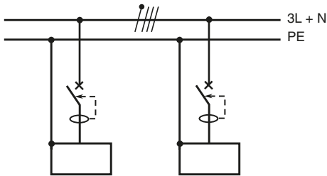
Fig. F30 RCD protection on TN systems with high earth-fault-loop impedance
