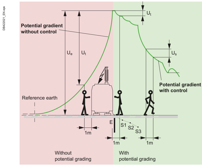
Fig. B13 Potential gradient control - EN50522 - Earthing of power installations exceeding 1 kV a.c.
