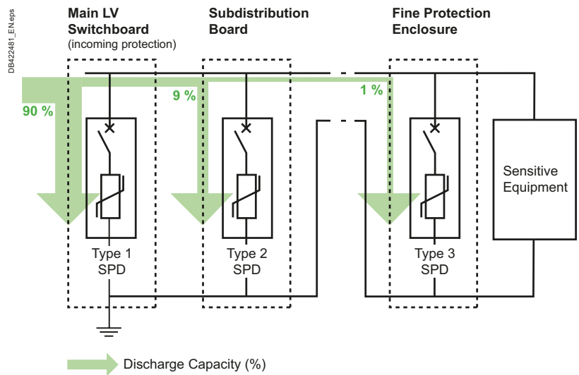
Fig. J22 Fine protection architecture Note: The Type 1 and 2 SPD can be combined in a single SPD
