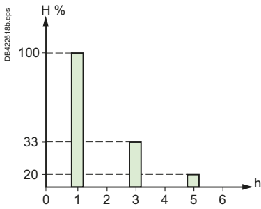
Fig. M9 Harmonic spectrum for a rectangular signal U(t)
