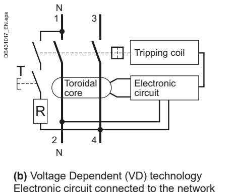
Fig. F47 The 2 technologies of RCDs
