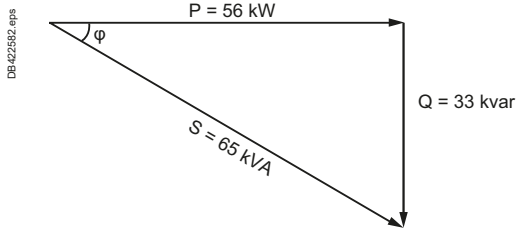
Fig. L4 Calculation power diagram
