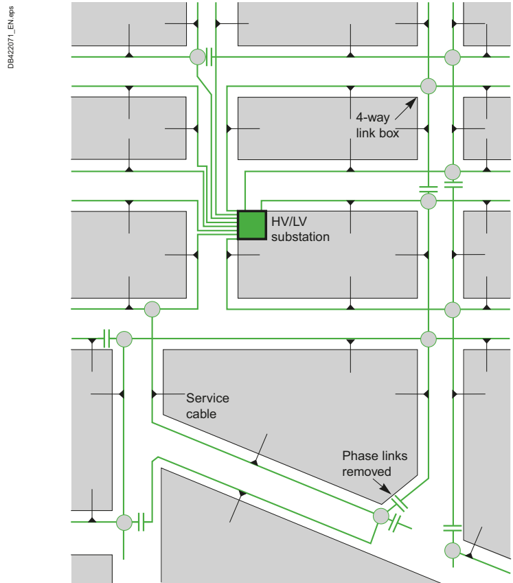
Fig. C4 Showing one of several ways in which a LV distribution network may be arranged for radial branched-distributor operation, by removing (phase) links
