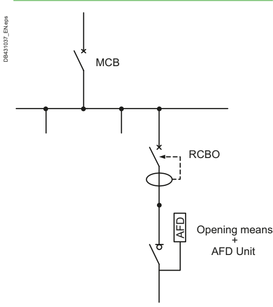
Fig. F91 AFDD unit with opening means installed in series with an RCBO
