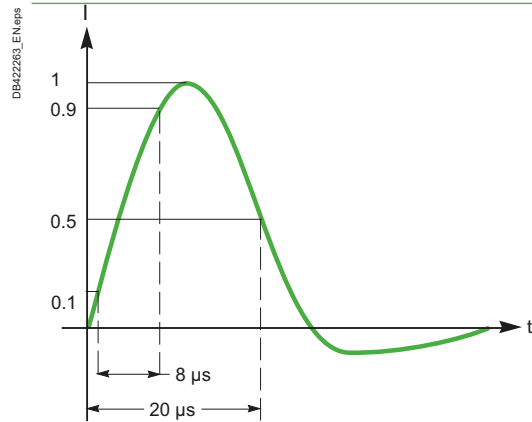
Fig. F55 Standardized current-impulse wave 8/20 μs
