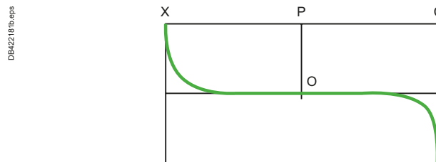
b) showing the effect on the potential gradient when (X) and (C) are widely spaced. The location of test electrode P is not critical and can be easily determined.
