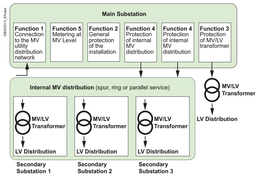
Fig. B4 Installation including several secondary substations supplied by an internal MV distribution
