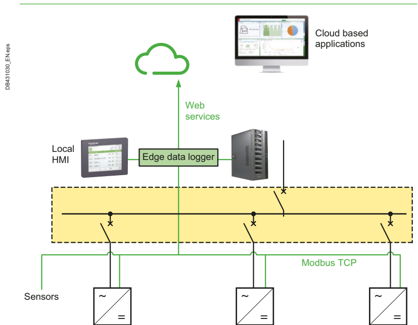
Fig. P31 Monitoring system for commercial PV installations
