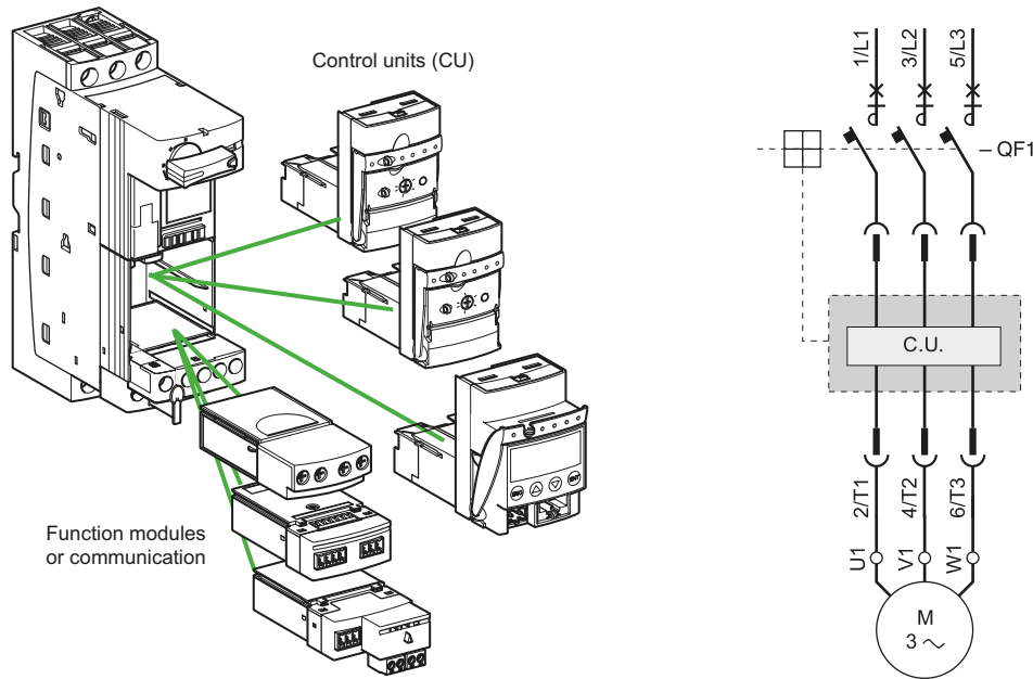
Fig. N86 Example of a CPS modularity (TeSys U starter controller by Schneider Electric)
