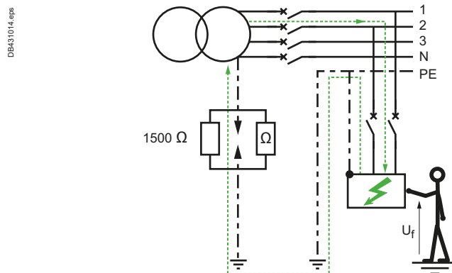
Fig. F32 Simplified circuit
