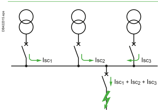
Fig. G34 Case of several transformers in parallel
