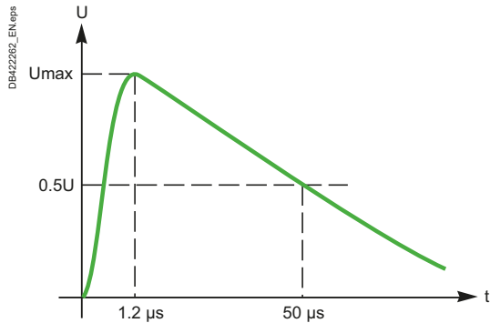
Fig. F54 Standardized 1.2/50 μs voltage transient wave
