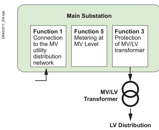
Fig. B2 Installation including a single MV/LV power transformer with metering at MV level
