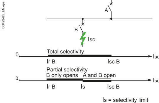
Fig. H49 Total and partial selectivity
