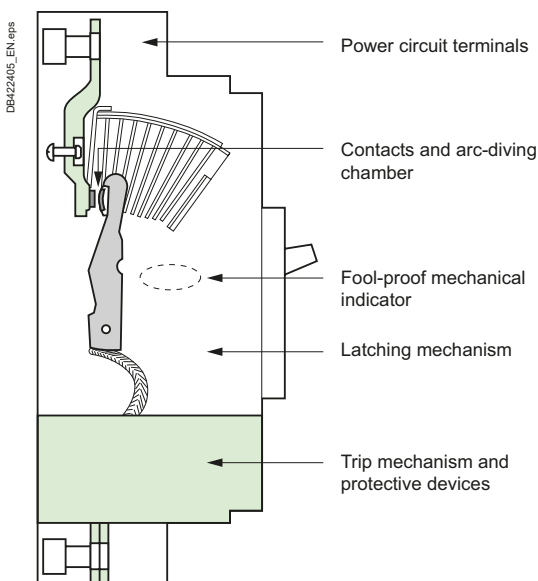
Fig. H21 Main parts of a circuit breaker
