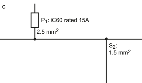
Fig. G7 Location of protective devices
