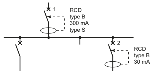
Fig. F64 Coordination between RCDs type B
