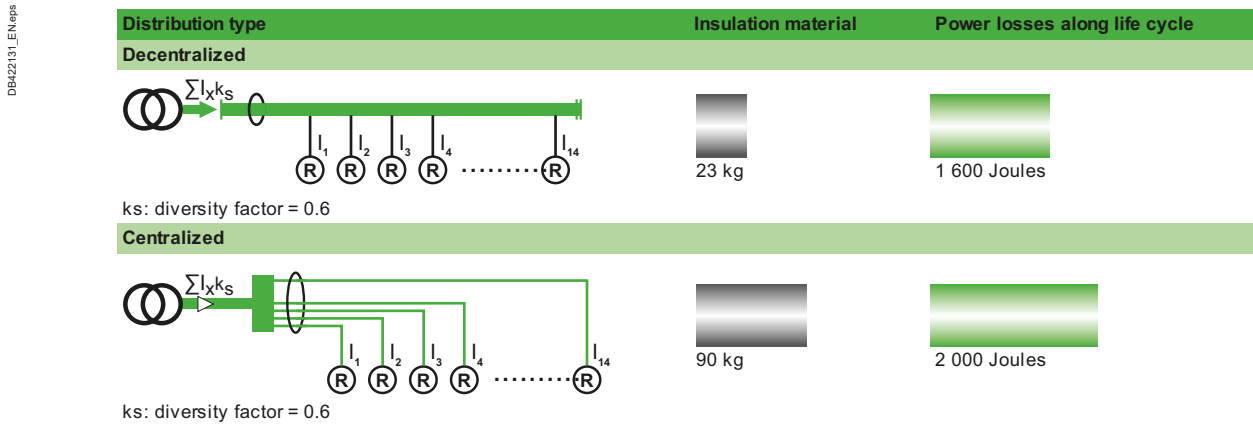
Fig. D17 Example of a set of 14 x 25A loads distributed along 34 meters (for busway, Canalis KS 250A)
