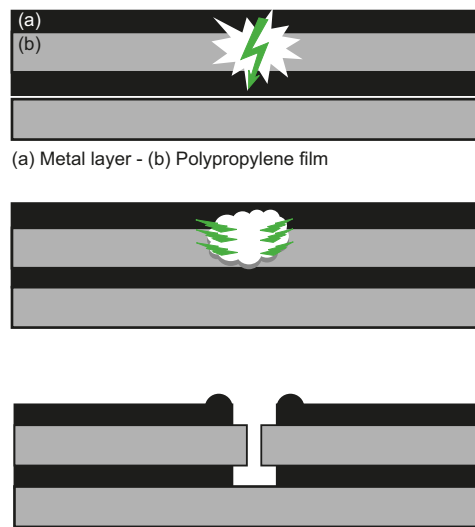
Fig. L35 Illustration of self-healing phenomena
