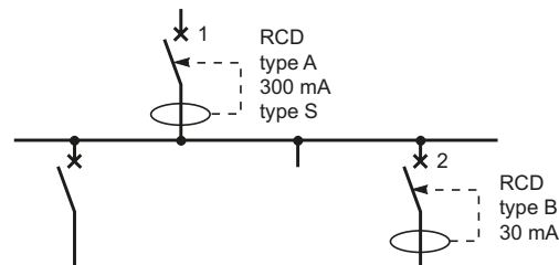
Fig. F65 Coordination between RCD type A and RCD type B
