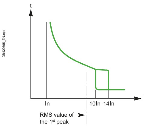
Fig. N35 Tripping characteristic of a Acti 9 curve D
