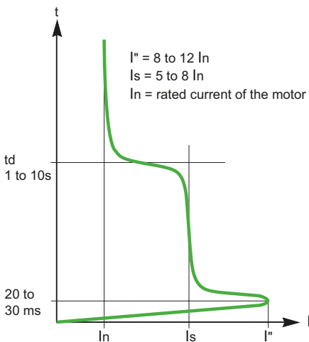
Fig. N74 Direct on-line starting current characteristics of an induction motor
