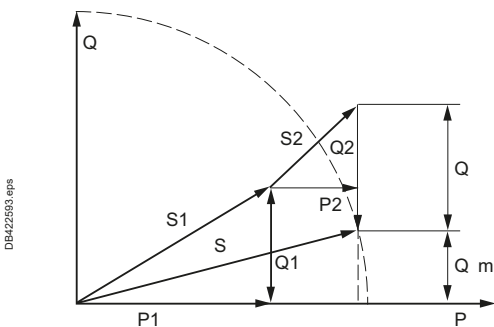
Fig. L19 Compensation Q allows the installation-load extension S2 to be added, without the need to replace the existing transformer, the output of which is limited to S
