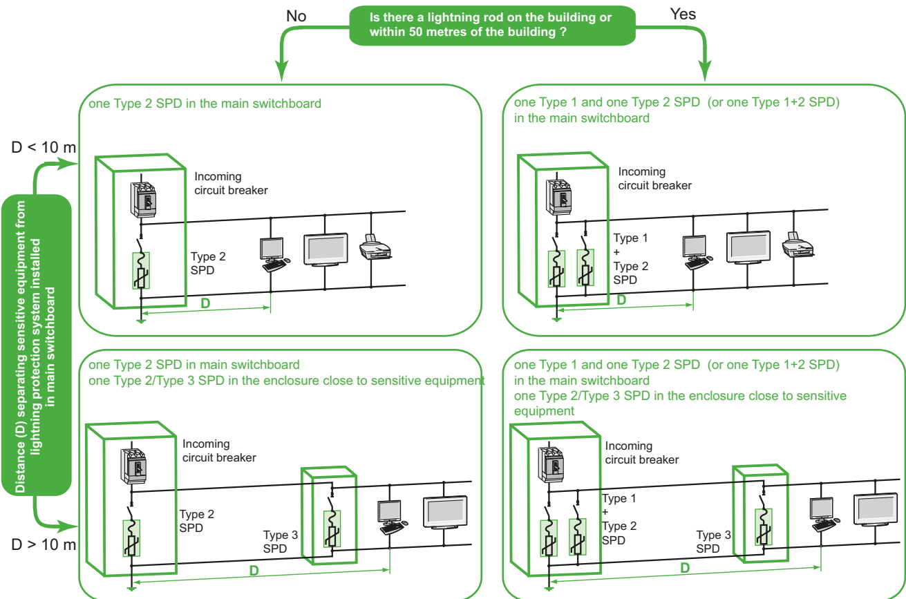
Fig. J21 The 4 cases of SPD implementation
