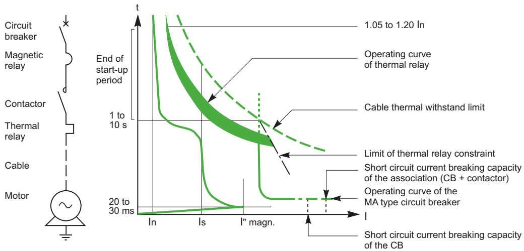
Fig. N85 Tripping characteristics of a circuit breaker + contactor + thermal relay
