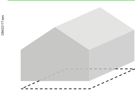
Fig. E20 Conductor buried below the level of the foundations, i.e. not in the concrete
