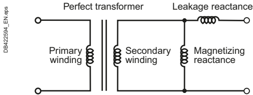
Fig. L20 Transformer reactances per phase
