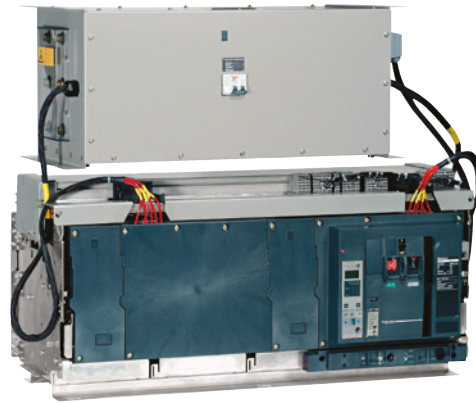
Fig. H58 Example of ultra rapid power circuit breaker: Masterpact UR (Schneider Electric)
