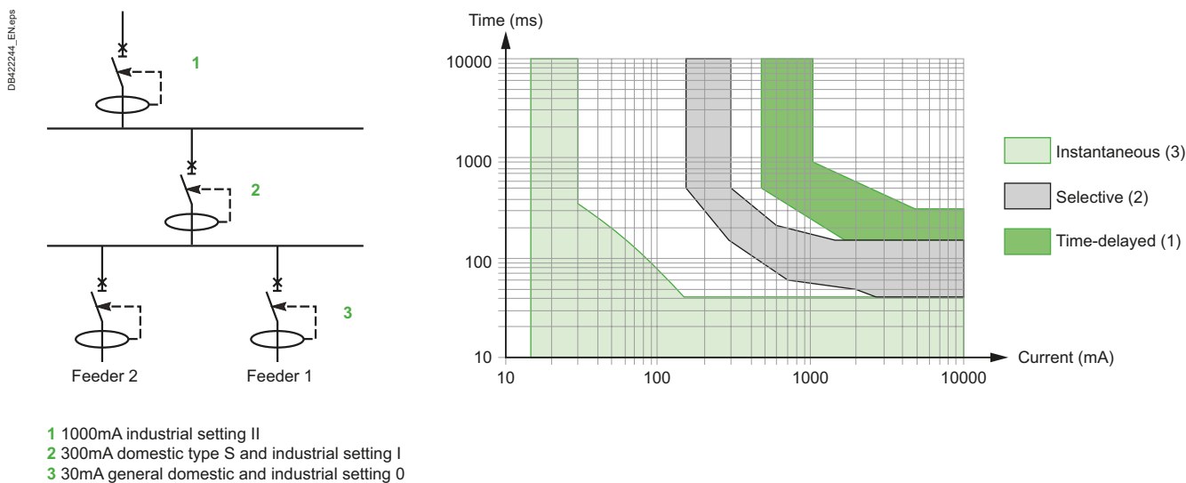
Fig. F61 Total selectivity at 3 levels
