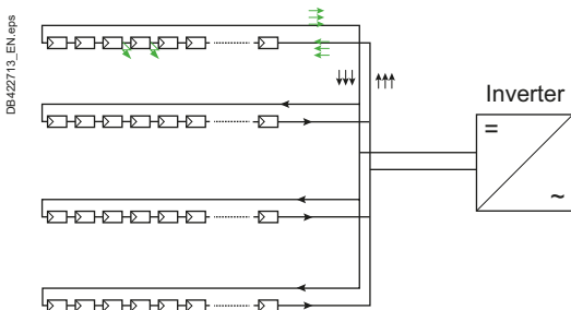
Fig. P12 Reverse current
