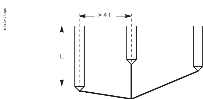
Fig. E21 Earthing rods connected in parallel
