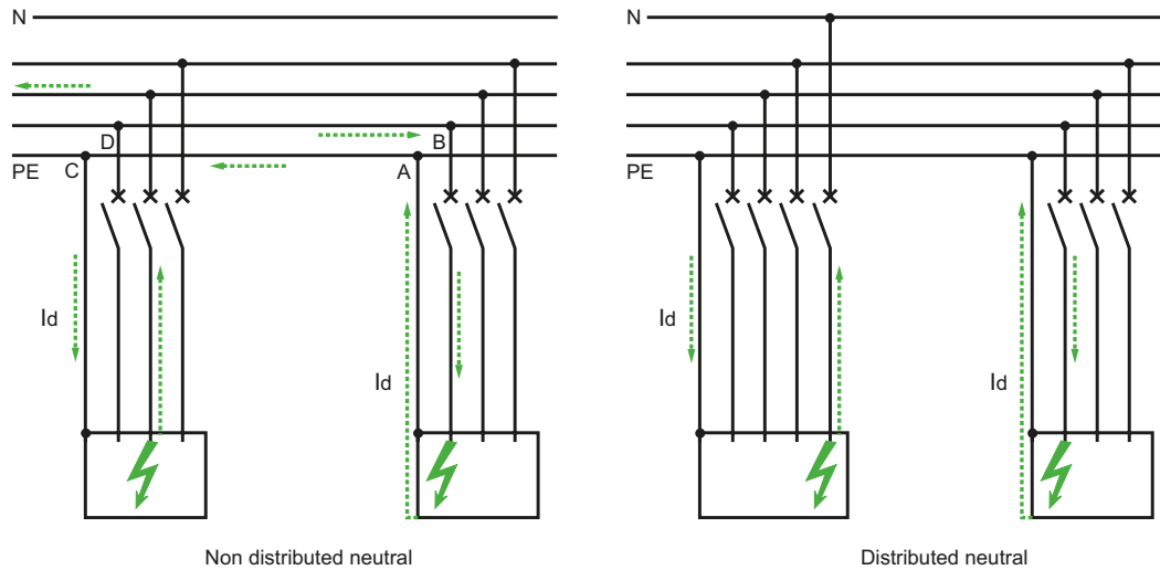
Fig. F39 Calculation of L_{max} for an IT-earthed system, showing fault-current path for a double-fault condition
