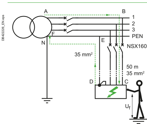
Fig. F18 Automatic disconnection in TN system
