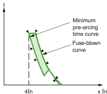
Fig. H11 Standardized zones of fusing for type aM fuses (all current ratings)
