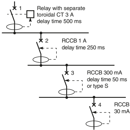
Fig. F63 Total selectivity at 3 or 4 levels
