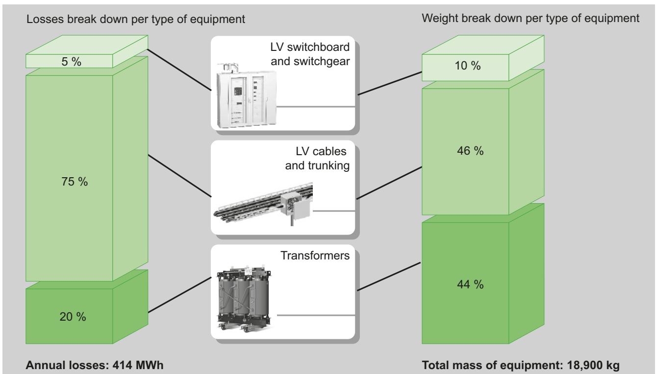
Fig. D28 Example of the break down of losses and the weight for each type of equipment
