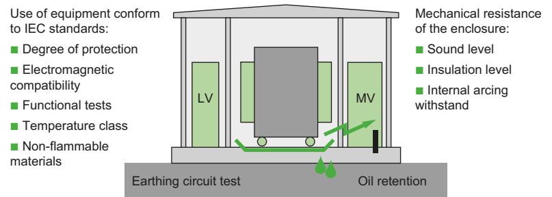
Fig. B49 Type tested substation according to IEC 62271-202
