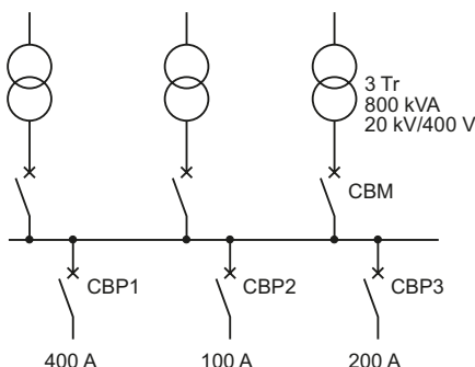
Fig. H45 Transformers in parallel
