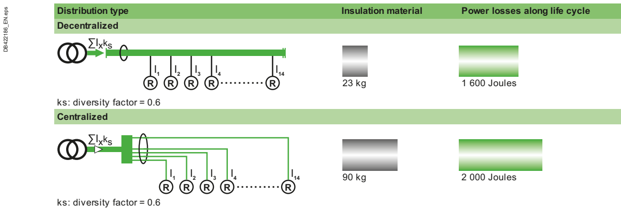
Fig. E46 Example of a set of 14 x 25A loads distributed along 34 meters (for busway, Canalis KS 250A)
