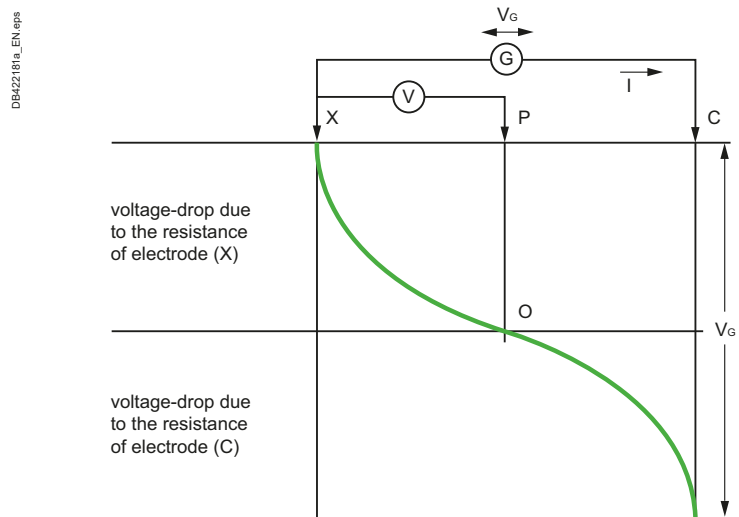
a) the principle of measurement is based on assumed homogeneous soil conditions. Where the zones of influence of electrodes C and X overlap, the location of test electrode P is difficult to determine for satisfactory results.
