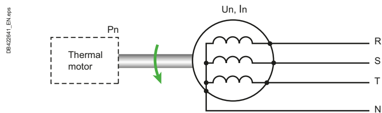
Fig. N2 Block diagram of a generator set
