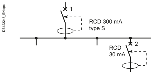
Fig. F62 Total selectivity at 2 levels
