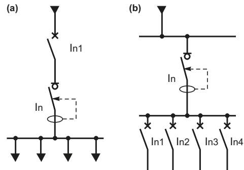
Fig. F60 Residual current circuit breakers (RCCBs)
