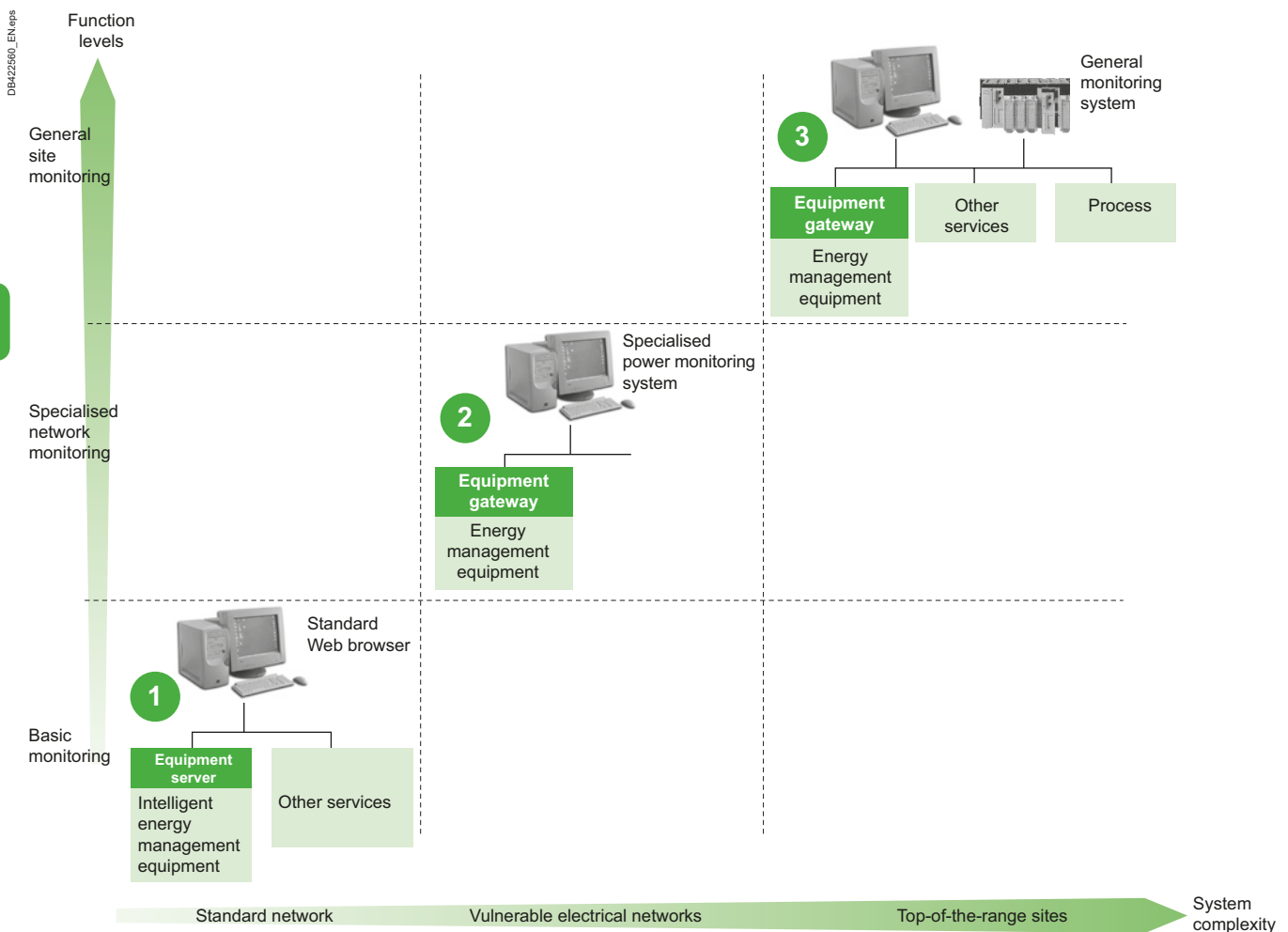
Fig. K27 Layout of a monitoring system
