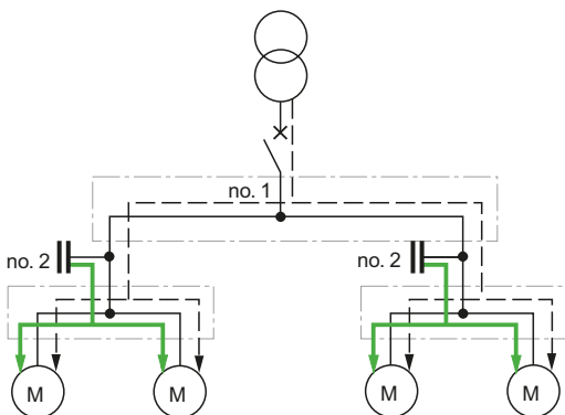
Fig. L15 Compensation by sector
