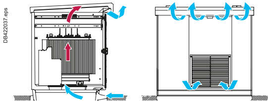
Fig. B42 Two different examples of HV/LV substation designs with natural ventilation, according to the layouts described in Fig. B48
