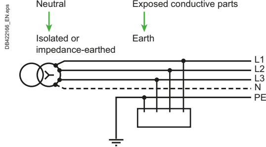
Fig. E8 IT system (isolated neutral)
