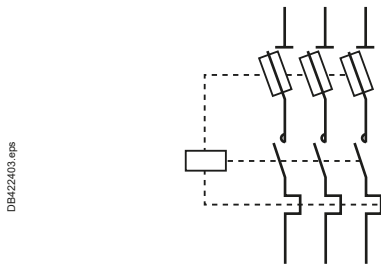
Fig. H17 Symbol for a fuse disconnecter + disconnector
