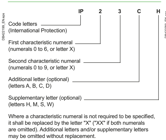
Fig. E66 IP Code arrangement
