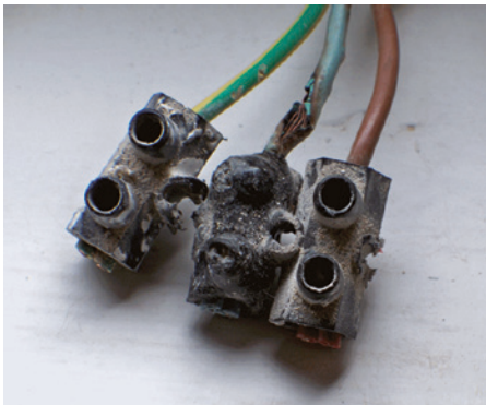
Fig. F84 Example of a carbonized connection
