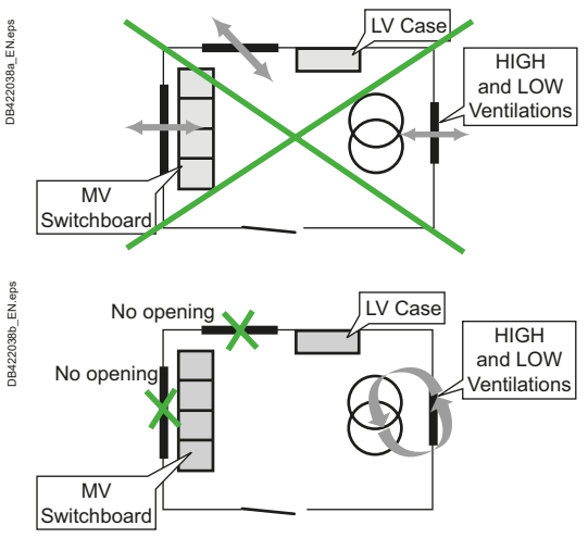
Fig. B44 Ventilation opening locations
