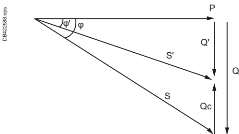
Fig. L10 Diagram showing the principle of compensation: Qc = P (\tan \phi - \tan \phi')
