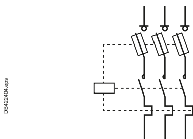
Fig. H18 Symbol for a fuse-switch disconnecter + disconnector
