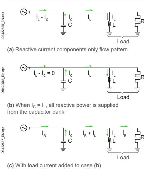
Fig. L9 Showing the essential features of power-factor correction
