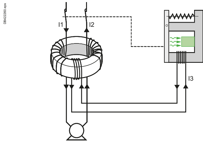
Fig. F46 Principle of RCD
