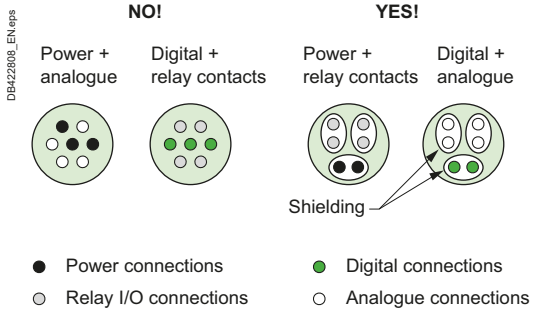
Fig. R42 Incompatible signals = different cables
