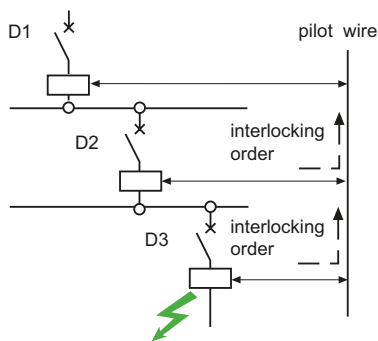
Fig. H55 Logic selectivity.
