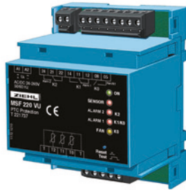
Fig. B20 Thermal relay for protection of dry type transformer (Ziehl)
