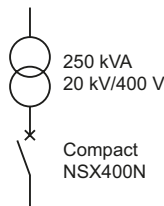
Fig. H43 Example of a transformer in a consumer's substation
