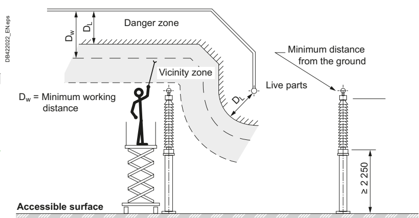
Fig. B15 Protection by placing live parts out of reach. The safety distances are fixed by IEC 61936
