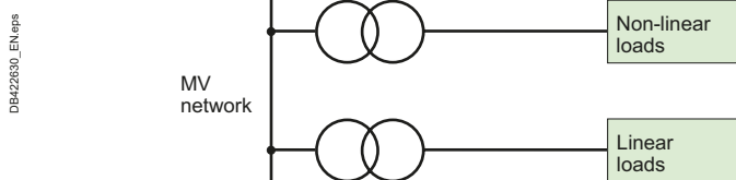
Fig. M26 Supply of non-linear loads via a separate transformer
